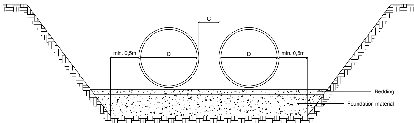
Figure 9. Distance between pipes in the same trench.
