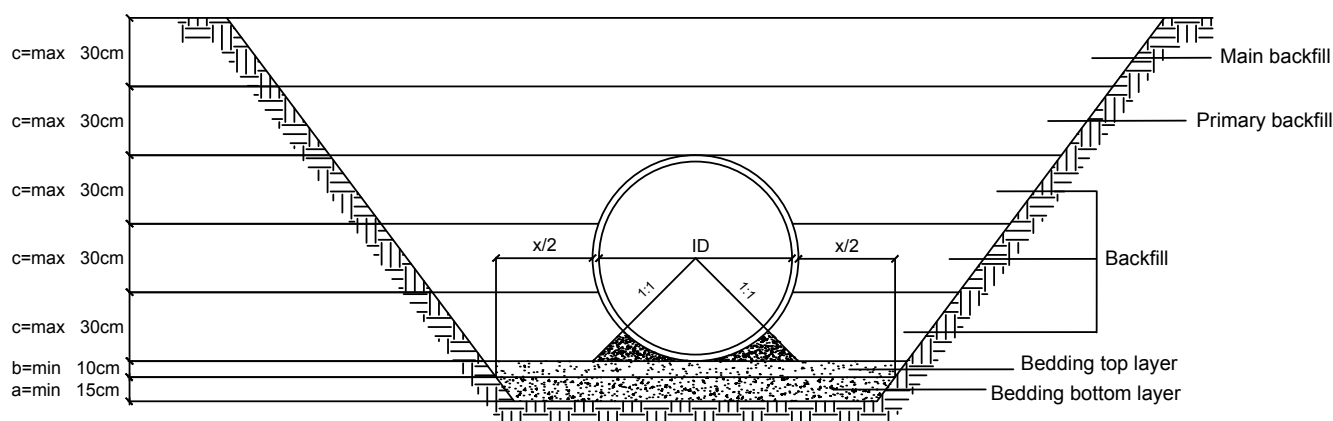
Figure 7. Laying the bedding and compacting the backfill when installing Pecor Quattro pipes.
