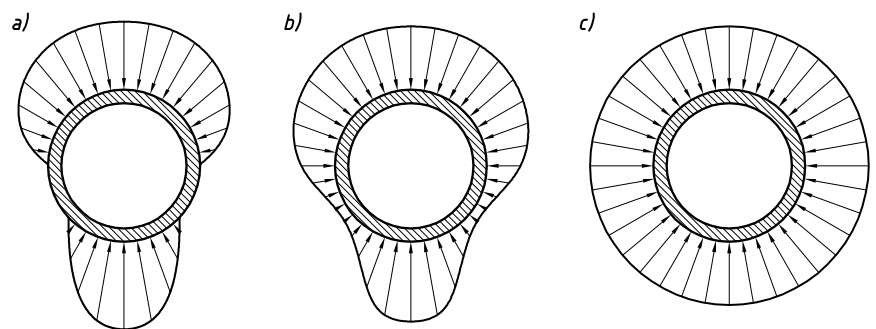
Figure 10. Load distribution in pipes: (a) rigid, (b) flexible, (c) perfectly flexible (under identical construction and loading conditions)
