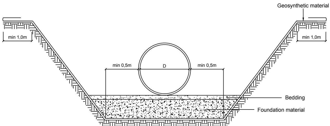
Figure 8. Pipe laying on low load-bearing capacity soils.
